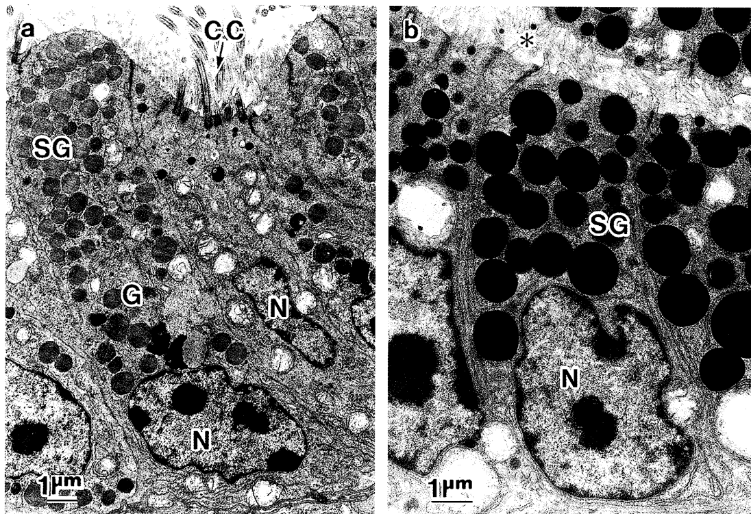
Fig. 2. Electron micrographs of the mucosa at the infundibulum. (a) The luminal epithelium consists of alternately distributed secretory cells and ciliated cells (CC). The apical cytoplasm of secretory cells is filled with electron-lucent secretory granules (SG). (b) The tubular gland consists exclusively of secretory cells possessing electron-dense secretory granules. The asterisk (*) indicates the glandular canal. G, Golgi complex; N, nucleus.
